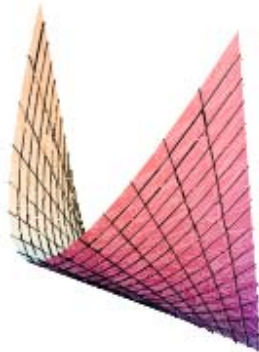
Figure 7: \sigma_4 : a = c = 0, b < 0
