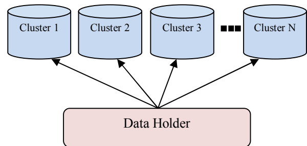
Fig.2. Multiparty clustering
