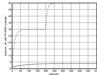
Figure 3 Process with decoupling ( Kravaris) with PI controller for level and pH process
